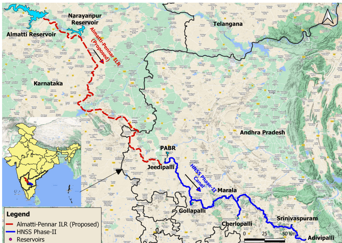
Optimal Alignment of Almatti-Pennar Inter-Linking Project.
